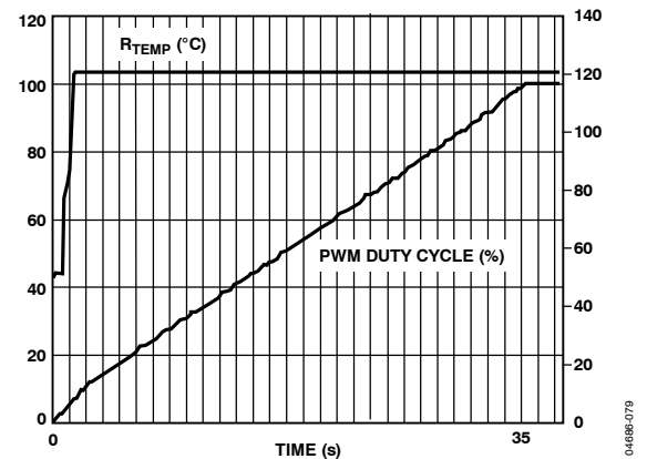
Figure 82. Enhanced Acoustics Mode with Ramp Rate = 1
