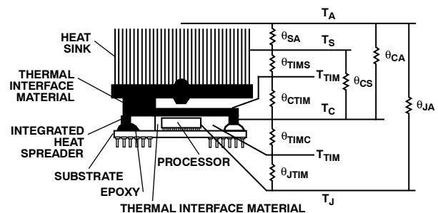
Figure 67. Thermal Model
